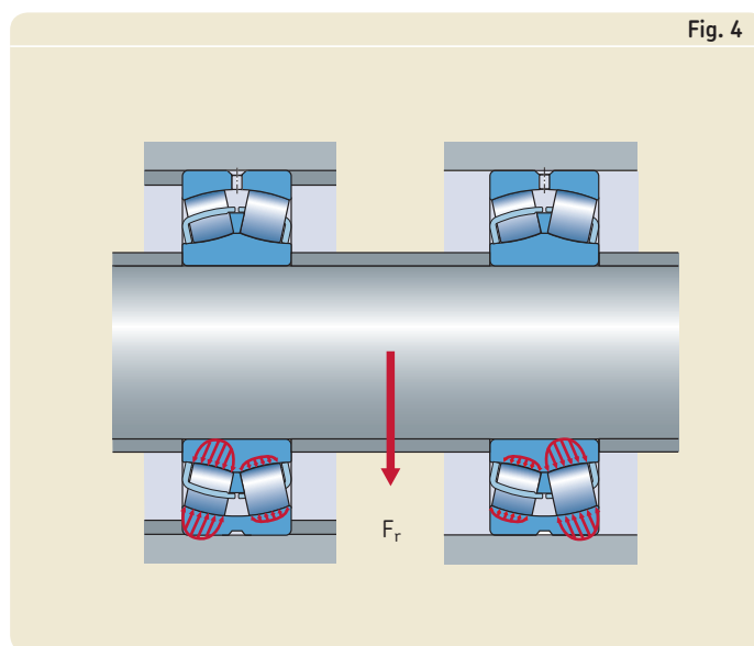
Uneven load distribution is caused by forces emanating from friction in the axial direction
