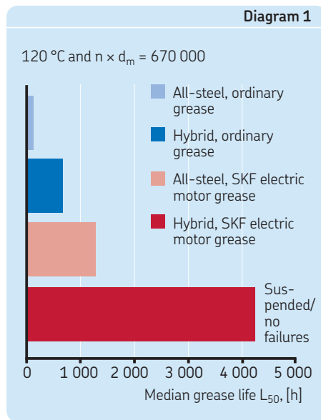
Grease life performance – test result where the grease life in SKF hybrid bearings is four times longer than in the corresponding all-steel bearings
