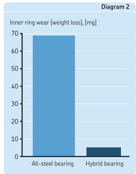
Wear performance under contaminated lubricant conditions
