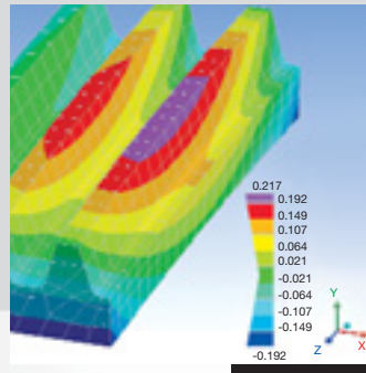
Thermal vertical deformation to 1/100 mm
