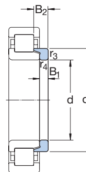
Angle ring
