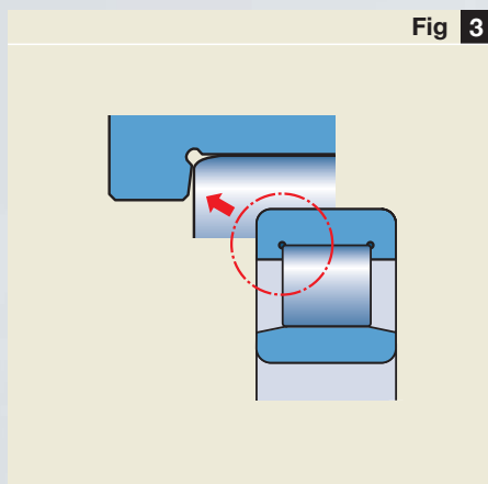
Opened flanges
