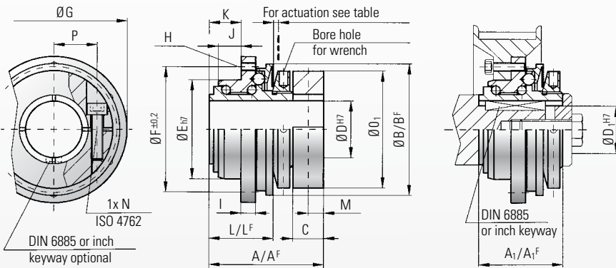
SK 1 with clamping hub
