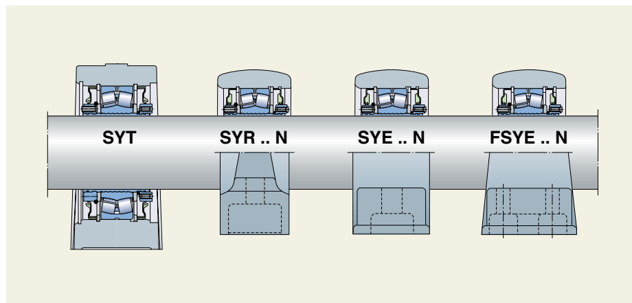
The ConCentra roller bearing unit designs
