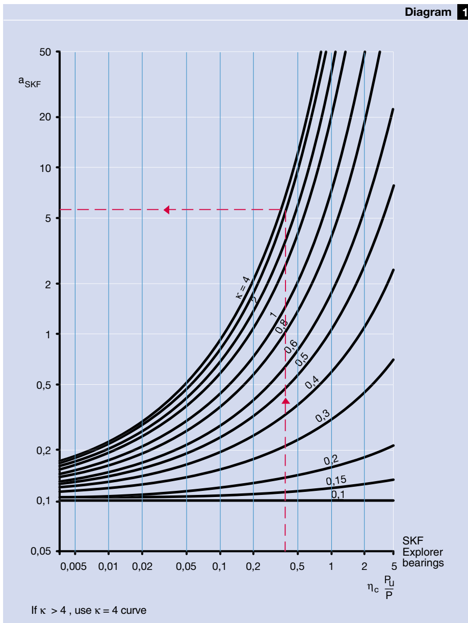
Factor a_{SKF} for SKF Explorer spherical roller bearings
