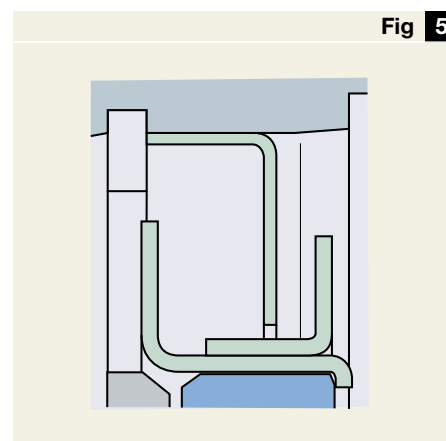
Labyrinth seal
