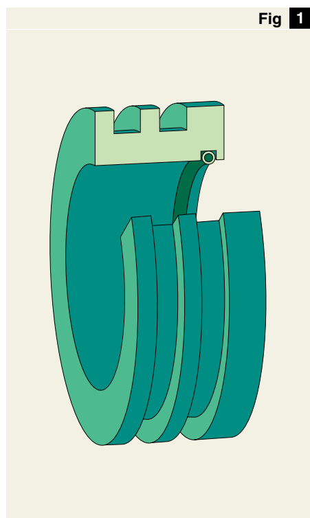
Labyrinth seal
