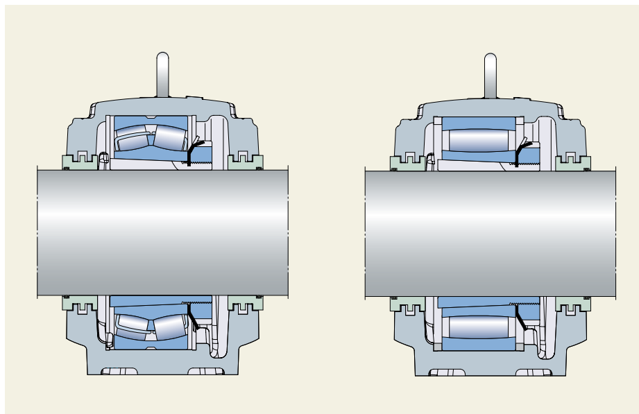
Bearings on adapter sleeves on smooth shafts
